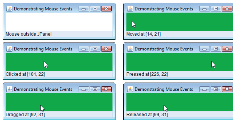
Fig. 26.29 | Testing MouseTrackerFrame.
