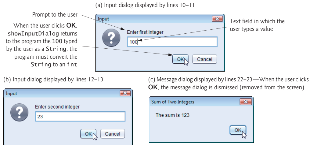
Fig. 26.2 | Addition program that uses JOptionPane for input and output. (Part 2 of 2.)
