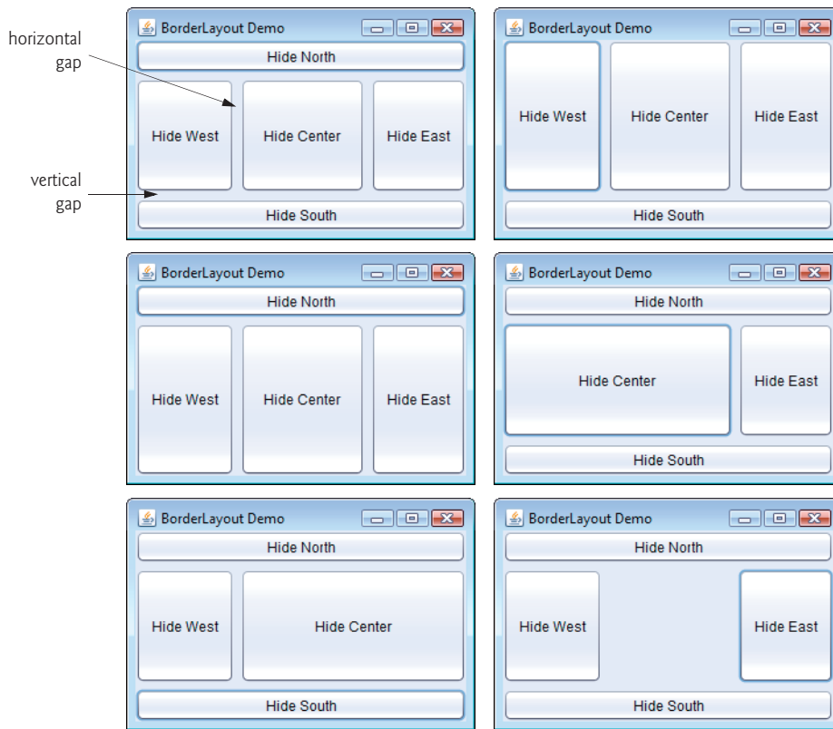
Fig. 26.42 | Testing BorderLayoutFrame. (Part 2 of 2.)
