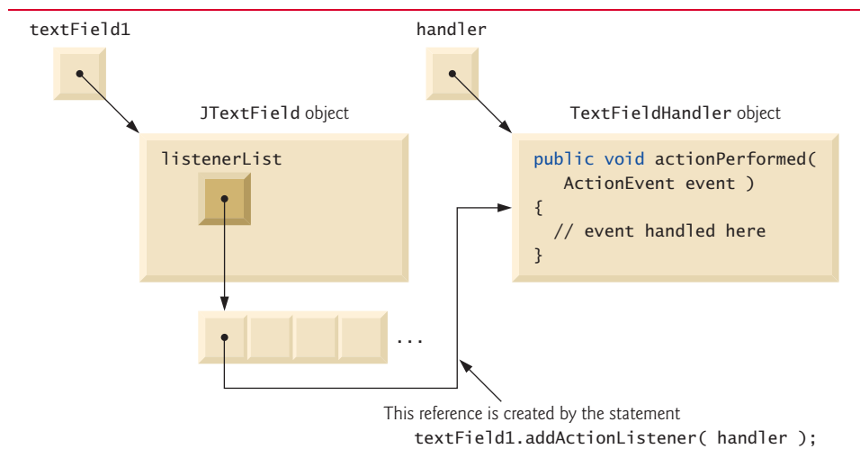
Fig. 26.13 | Event registration for JTextField textField1 .
