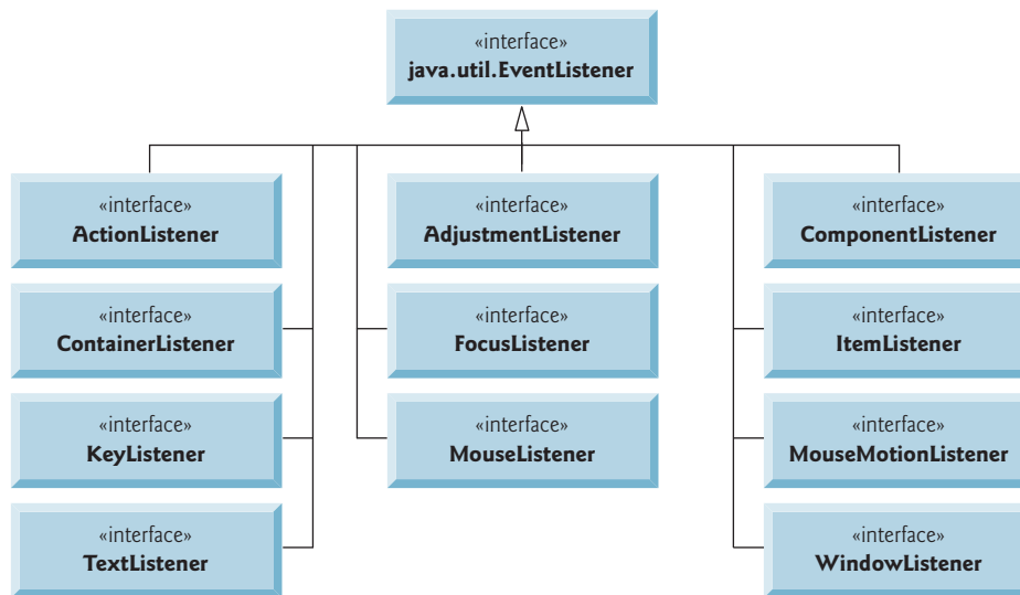
Fig. 26.12 | Some common event-listener interfaces of package java.awt.event .
