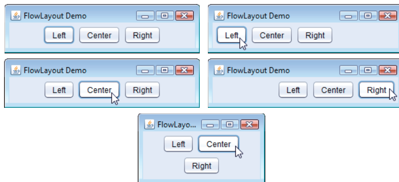
Fig. 26.40 | Testing FlowLayoutFrame.
