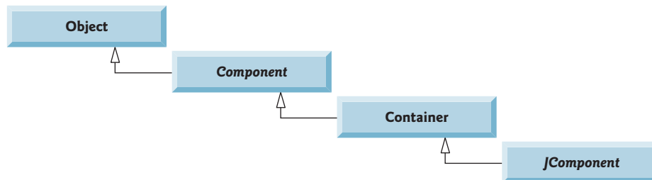
Fig. 26.5 | Common superclasses of the lightweight Swing components.
