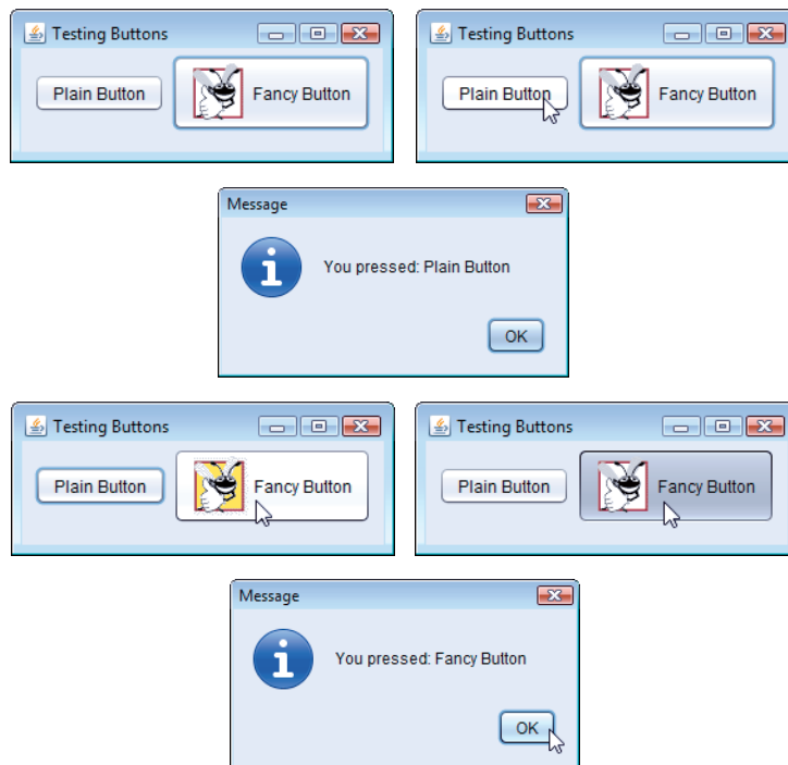
Fig. 26.16 | Testing ButtonFrame.
