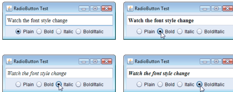
Fig. 26.20 | Testing RadioButtonFrame .
