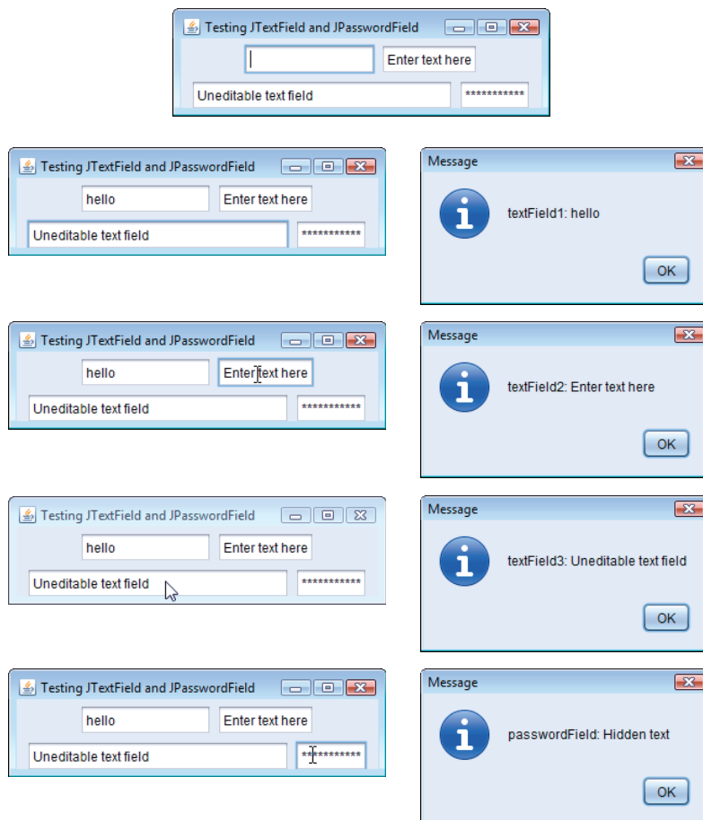
Fig. 26.10 | Testing TextFieldFrame.
