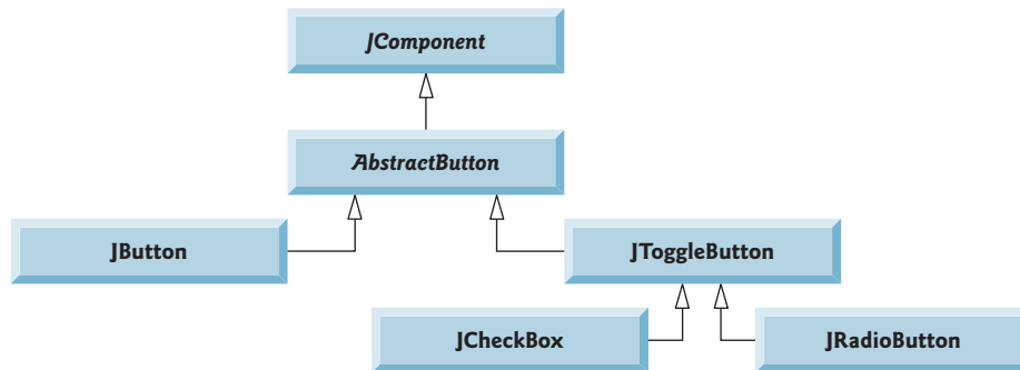
Fig. 26.14 | Swing button hierarchy.
