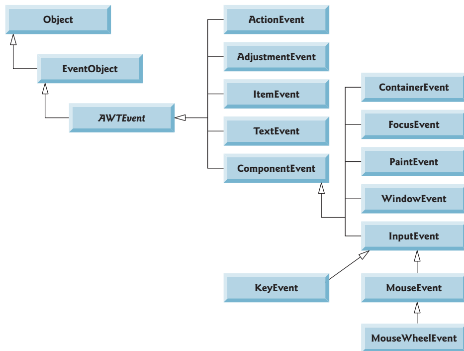
Fig. 26.11 | Some event classes of package java.awt.event .
