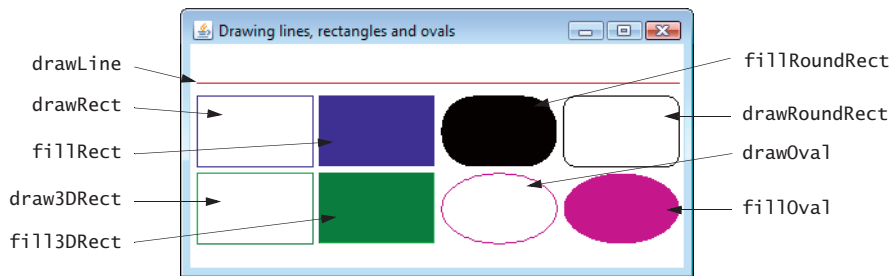
Fig. 27.19 | Testing LinesRectsOvalsJPanel.
