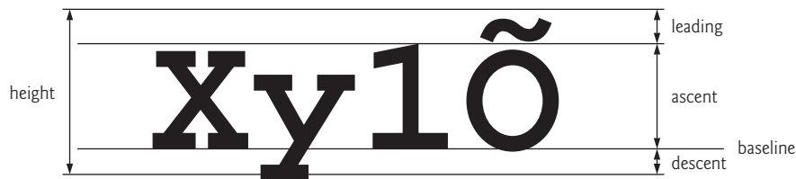
Fig. 27.13 | Font metrics.
