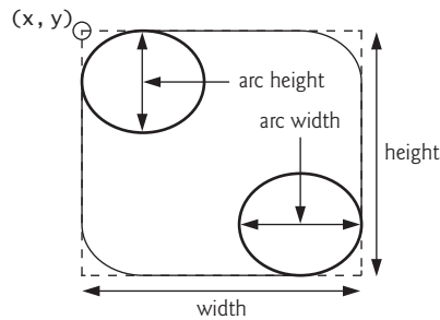
Fig. 27.20 | Arc width and arc height for rounded rectangles.
